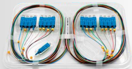
Splitter 1X16 SC/UPC
