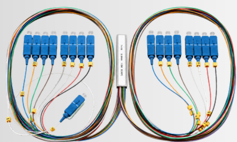
Splitter 1X16 SC/UPC
