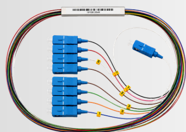
Splitter 1X8 SC/UPC
