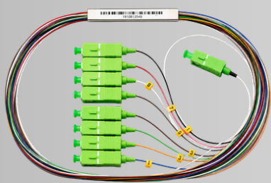
Splitter 1X8 SC/APC
